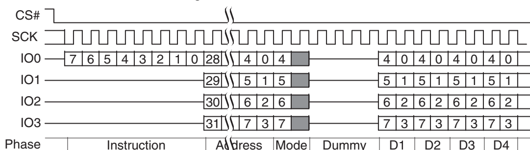
Figure 3.11 Quad I/O Command
