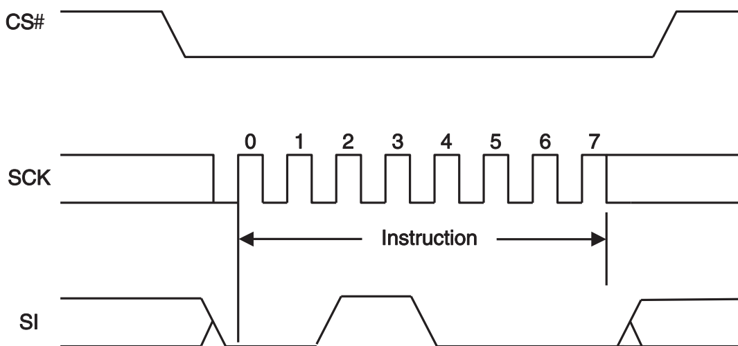
Figure 9.14 Clear Status Register (CLSR) Command Sequence
