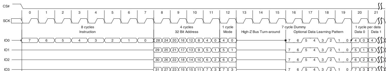
Figure 9.52 DDR Quad I/O Read Initial Access (4-byte Address, EEh or EDh [ExtAdd=1], EHPLC=01b)
