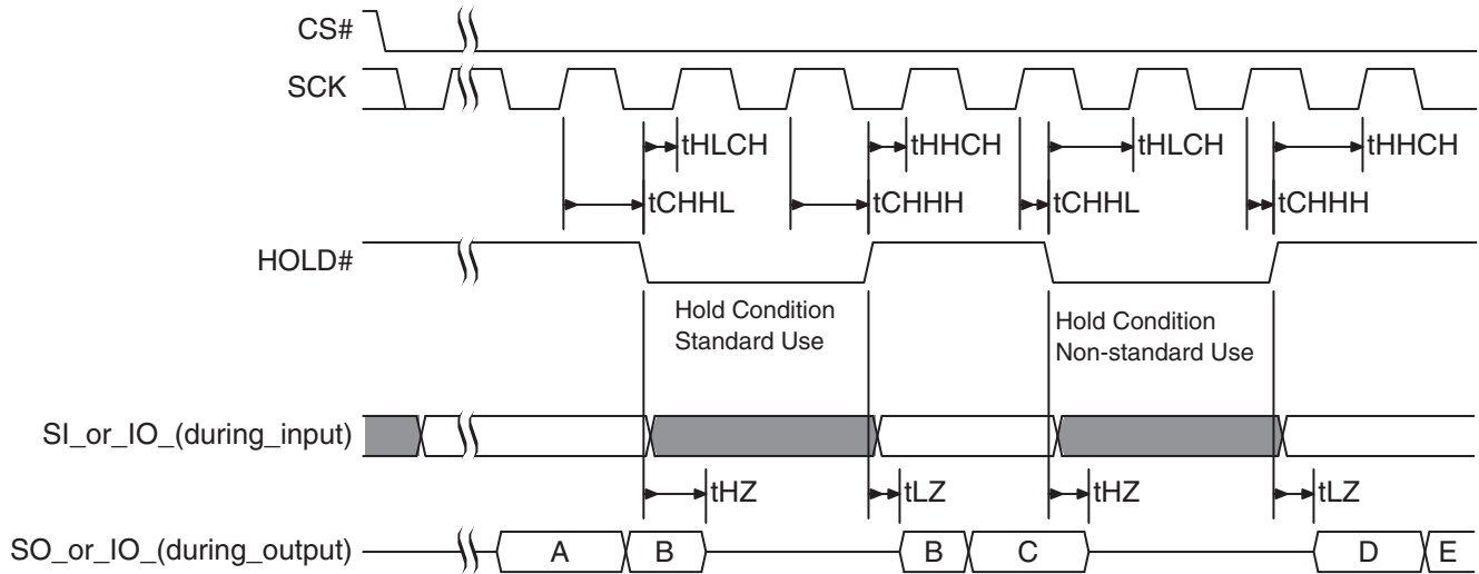
Figure 5.12 Hold Timing
