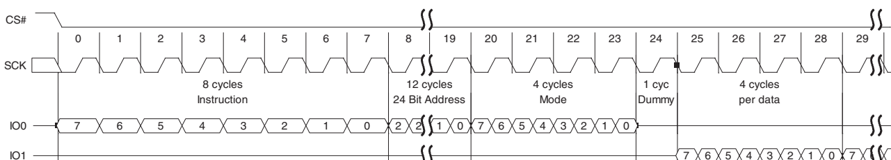
Figure 9.42 DDR Fast Read Initial Access (3-byte Address, 0Dh [ExtAdd=0, EHPLC=11b])
