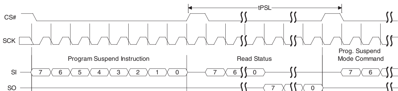
Figure 9.60 Program Suspend Command Sequence
