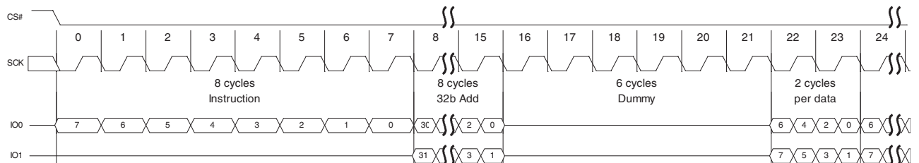
Figure 9.49 DDR Dual I/O Read (4-byte Address, BEh or BDh [ExtAdd=1], HPLC=00b)
