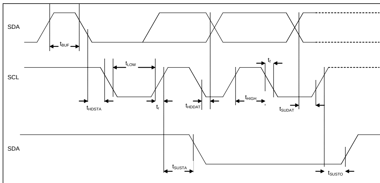
Figure 25: I 2 C timing diagram
